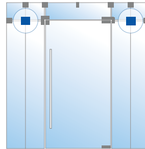
PF2HP Top Door Patch Fitting With Matching Plate
