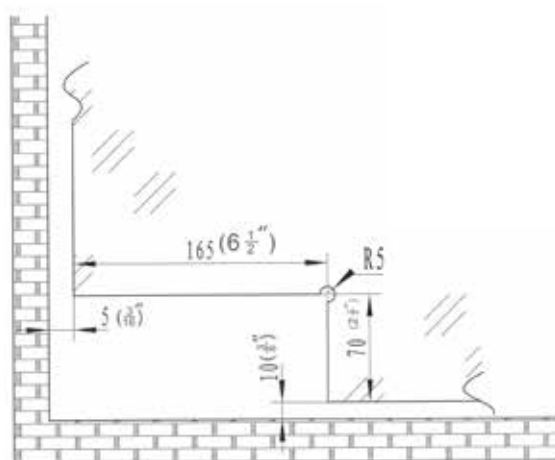
CFH100 Hydraulic Patch Fitting
