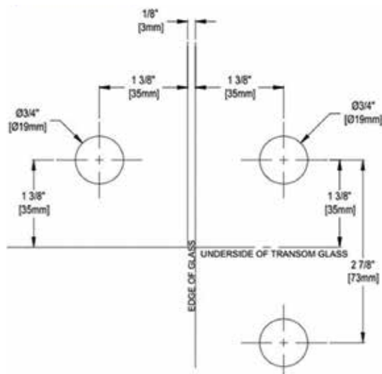
CFH105 Hydraulic Patch Fitting
