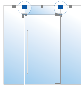
PF610 Sidelite Mounted Transom Patch With Door Stop
