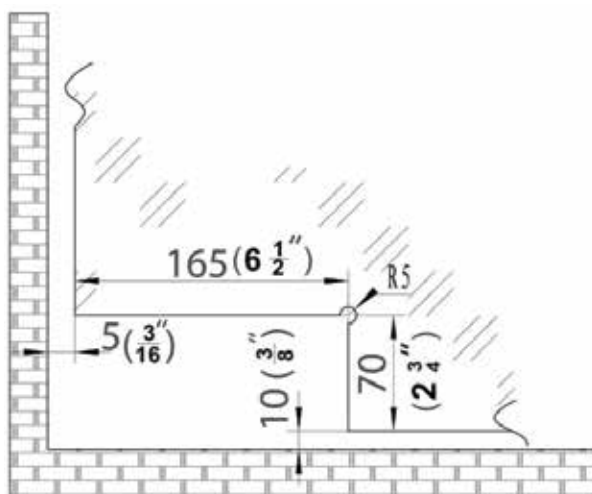
CFHP100 Hydraulic Patch Fitting
