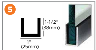
E3UC15X1 1-1/2 x 1 Channel
